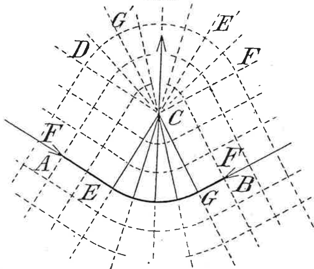
3. (Fig. 4.) Constructions similar to that of figs. 2 & 3 give the minimum frames for three forces, two of which are
